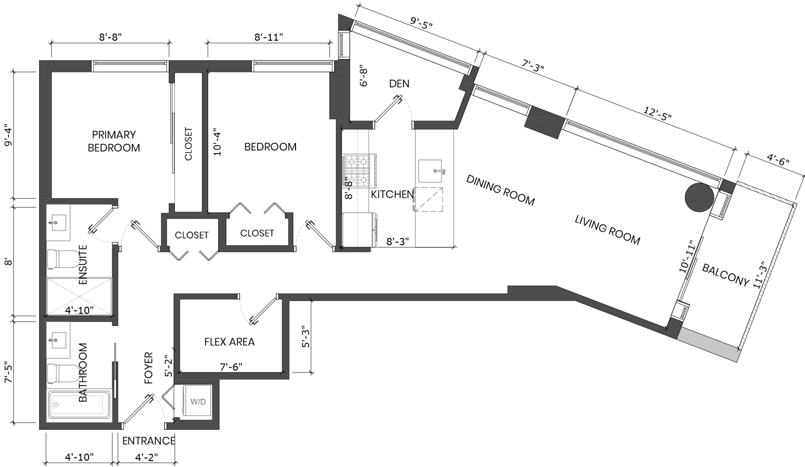
MAIN FLOOR PLAN Ceiling Height: 8'-6"
