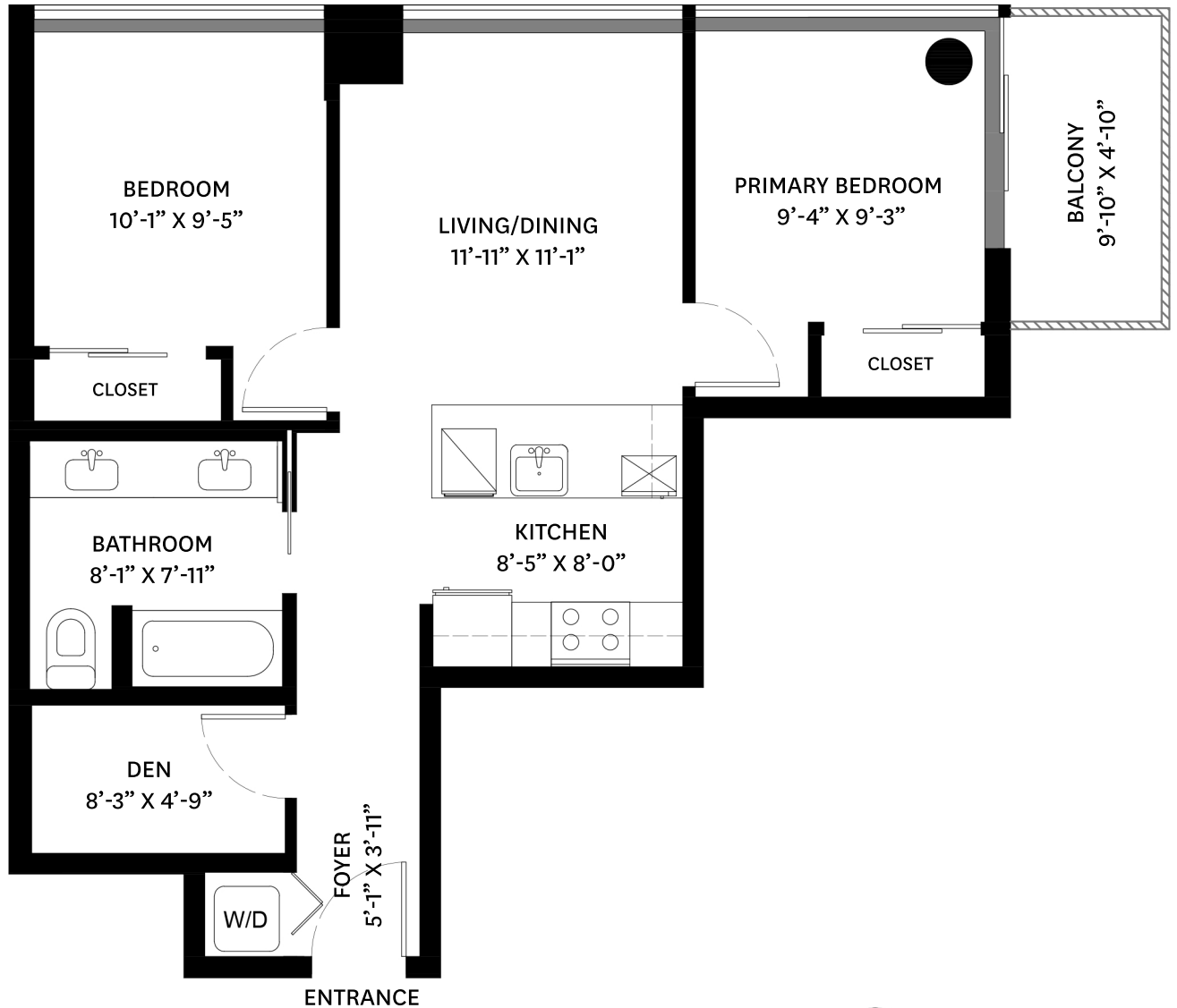
MAIN FLOOR PLAN Ceiling Height 8'-0"
