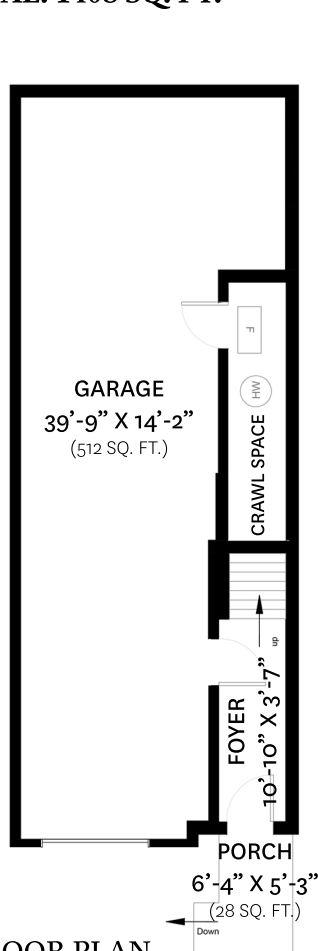
LOWER FLOOR PLAN Ceiling Height: 8'-11"
