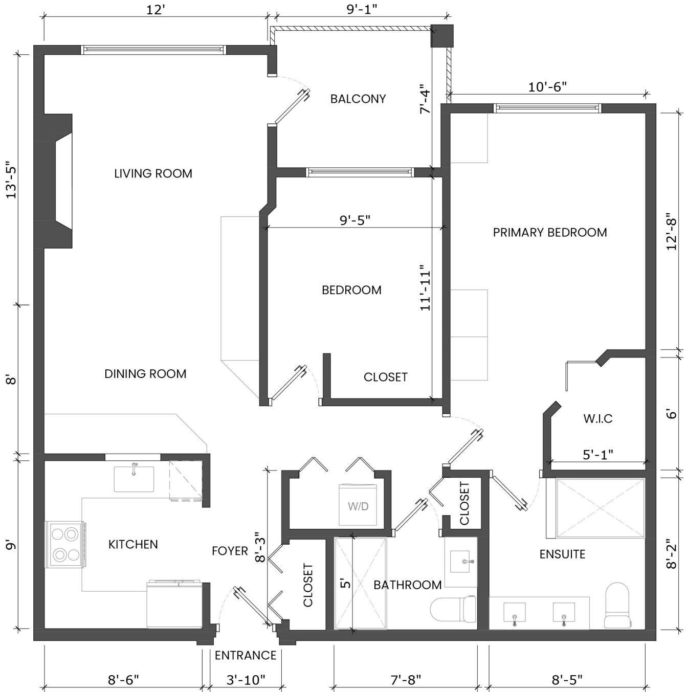
MAIN FLOOR PLAN Ceiling Height: 9'-0"
